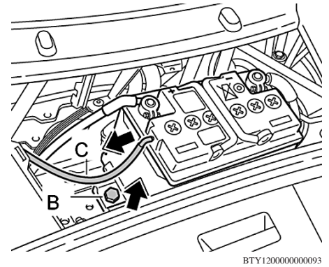
Fig. 2 Battery removal
