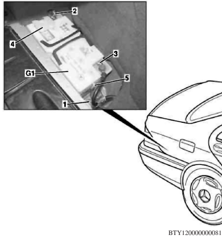
Fig. 1 Battery removal
