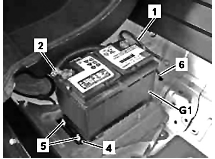
Fig. 2 Battery removal. P98 Black Series
