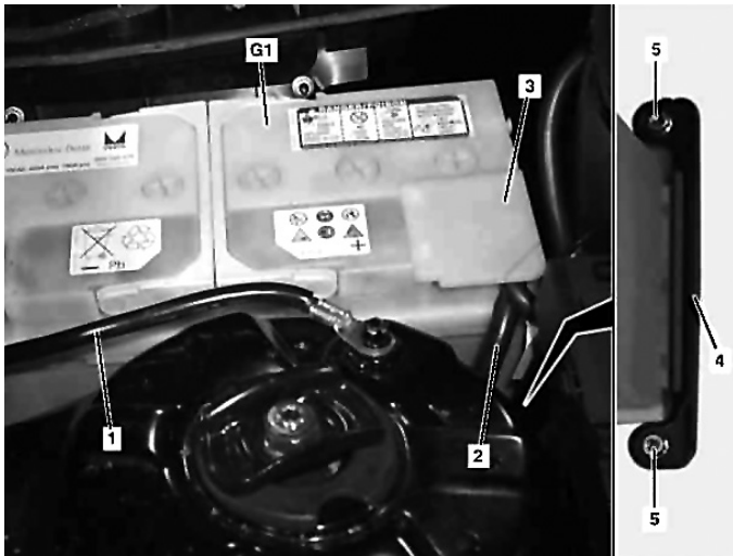
Fig. 1 Battery removal. Less P98 Black series
