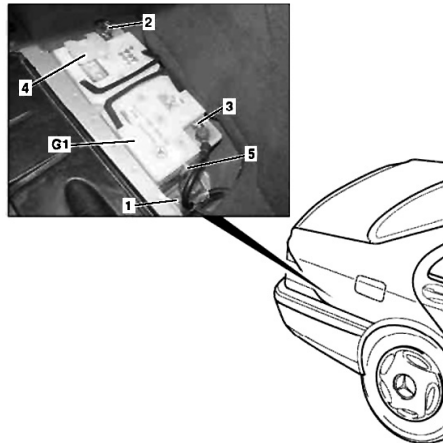
Fig. 1 Battery removal
