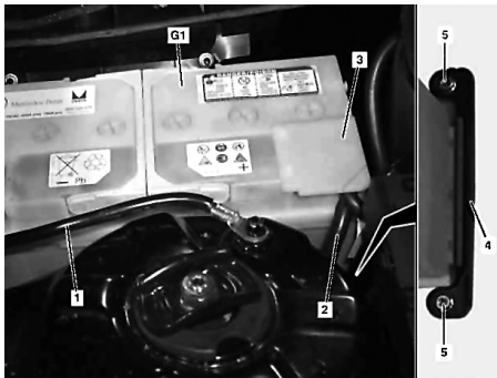
Fig. 1 Battery removal. Less P98 Black series
