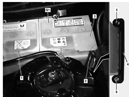
Fig. 1 Battery removal
