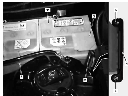
Fig. 1 Battery removal
