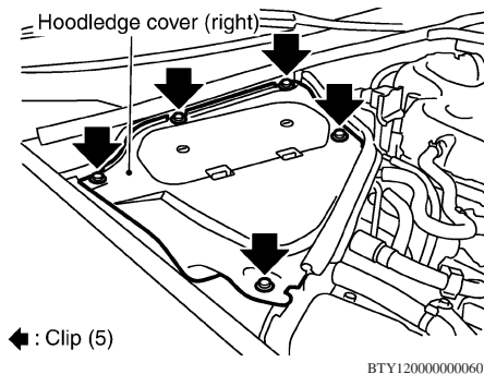
Fig. 1 Righthand hoodledge cover removal
