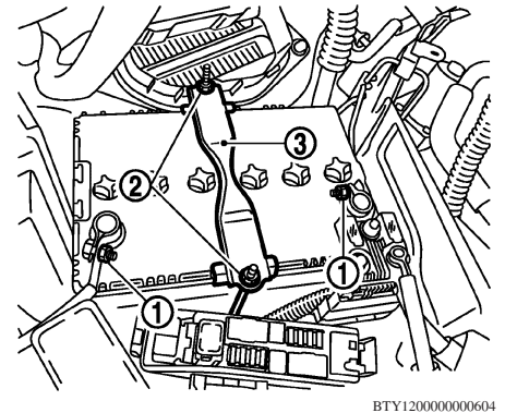
Fig. 2 Battery removal
