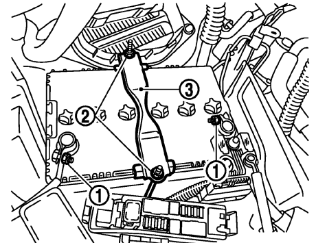
Fig. 2 Battery removal
