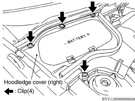
Fig. 1 Righthand hoodedge cover removal
