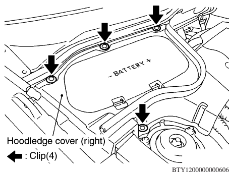
Fig. 1 Righthand hoodledge cover removal
