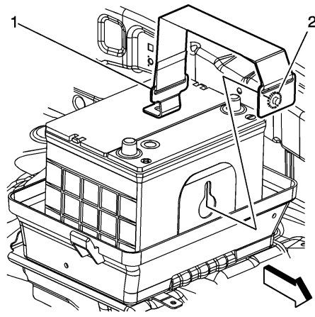
Fig. 4 Battery strap removal from battery tray bracket stopper
