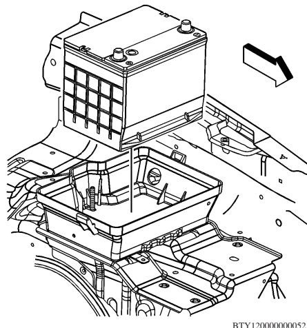
Fig. 6 Battery removal
