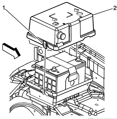
Fig. 3 Upper battery box removal
