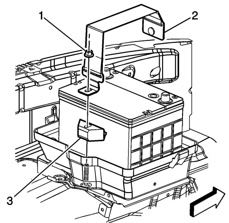
Fig. 5 Battery tray strap & hold down retainer removal
