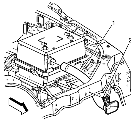
Fig. 2 Battery vent duct removal
