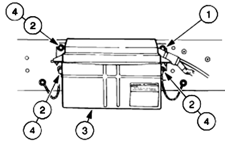
Fig. 3 Secondary battery removal
