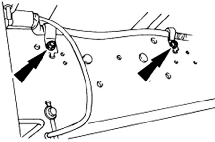
Fig. 2 Secondary battery cable harness removal
