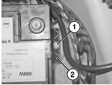
Fig. 5 Battery removal
