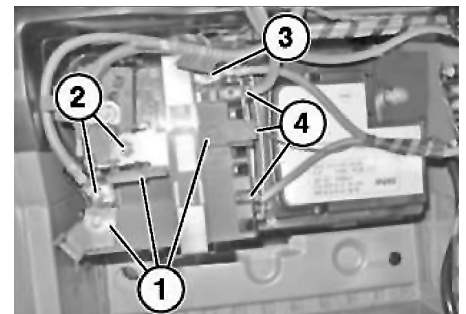
Fig. 2 Power distributor connector removal
