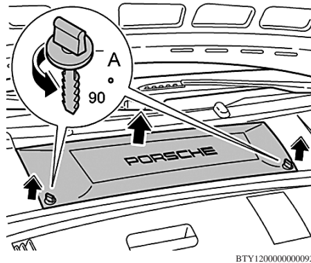
Fig. 1 Battery access cover
