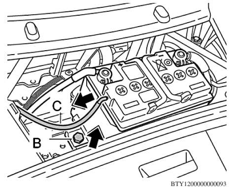
Fig. 2 Battery removal
