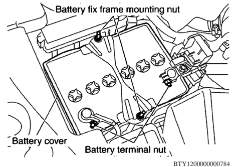
Fig. 1 Battery removal
