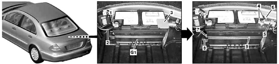
Fig. 1 Primary battery removal. Sedan
