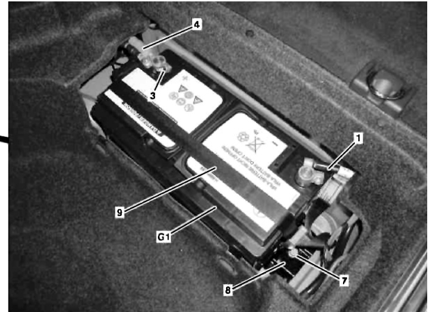
Fig. 4 Primary battery removal. Wagon
