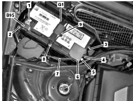
Fig. 1 Battery removal
