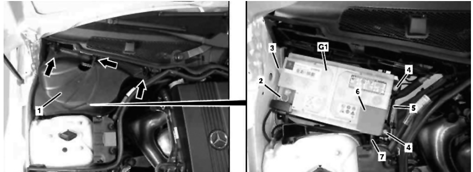
Fig. 1 Battery removal
