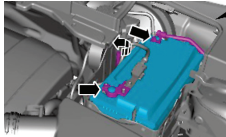
Fig. 1 Battery removal (Part 1 of 2)
