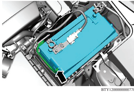
Fig. 1 Battery removal (Part 2 of 2)
